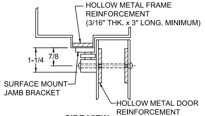
SIDE VIEW CROSS SECTION
